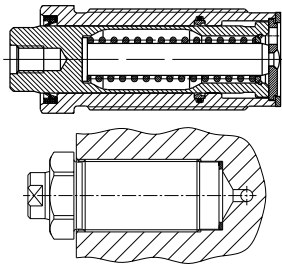
Threaded-body cylinder with locking piston (page 2)
